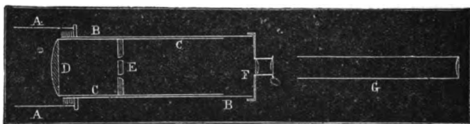
FIG. 46.—The annulus is viewed and brought to focus by looking through apertures in the side of the tubes. A, sliding eye-tube of telescope ; B, tube screwing into eye-tube ; C, tube sliding inside B, and carrying lens D and diaphragm E ; F, lenses bringing image of diaphragm to a focus at the place generally occupied by the slit of the spectroscope ; G, collimator of spectroscope.
