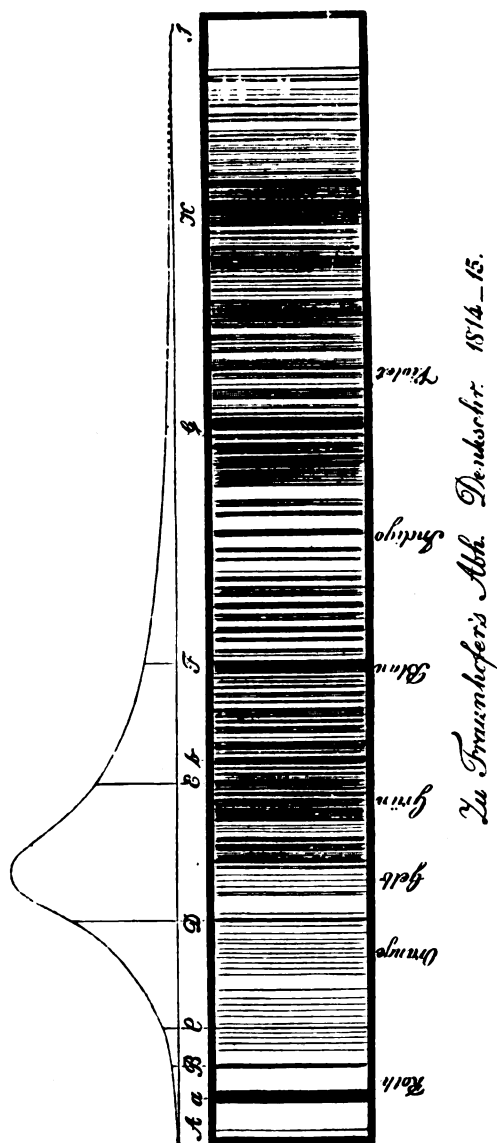
FIG. 6.—Reduced copy of Fraunhofer's map.
