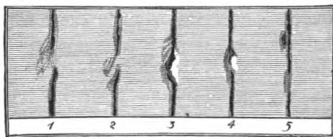
FIG. 56.—Contortions of F line on disc. 1 and 2, rapid downrush and increasing temperature ; 3 and 4, uprush of bright hydrogen and downrush of cool hydrogen ; 5, local downrushes associated with hydrogen at rest.
