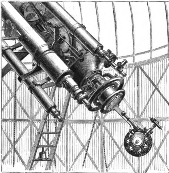
FIG. 37.—The eyepiece end of the Newall refractor (of 25 inches aperture) with spectroscope attached.
