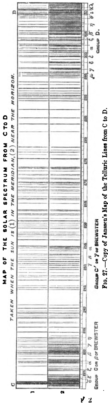
FIG. 26.—The Telluric Lines. Taken from the Atlas to Ångström's Spectre Normal . The observations shown extend over the whole of the visible spectrum. The red part of the spectrum is to the left.
