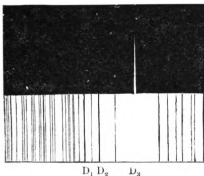
FIG. 42.—Line D_2 (yellow), with radial slit.
