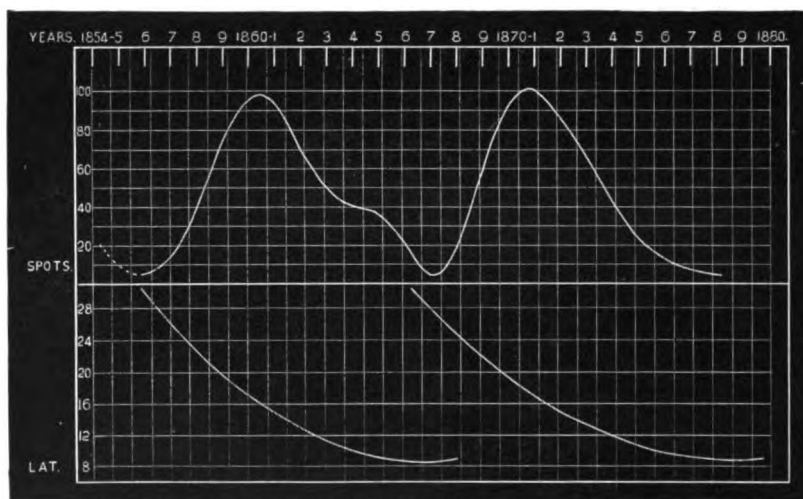
FIG. 130.—Combination of Spörer's curves.
