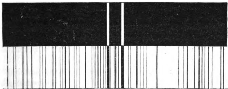
FIG. 24.—Diagram showing the solar spectrum and the bright double line \text{D} of sodium.
