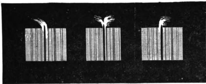
FIG. 55.—Contortions of the hydrogen lines. The right-hand side of each diagram is the most refrangible.
