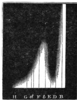
FIG. 19.—Absorption of sunlight by various thicknesses of a solution of potassic permanganate (Gladstone).
