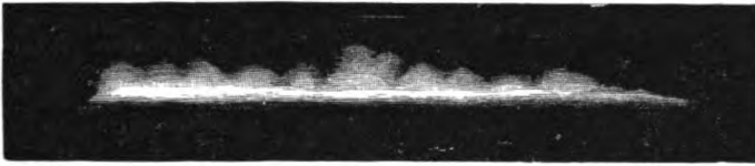
FIG. 48.—Edge of chromosphere (billowy).
