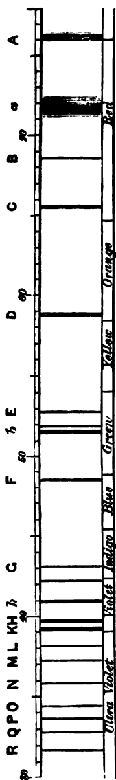
Fig. 78.—Wave-length map of the solar spectrum. The visible portion extends from A to K. The portion that could be photographed in 1874 extends from b to E.
