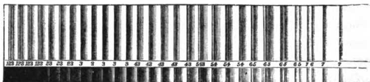
FIG. 71.—Fluted spectrum of iodine. (Thalén.)
