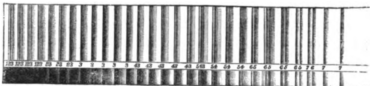
FIG. 21.—Absorption spectrum of iodine (Thalén).
