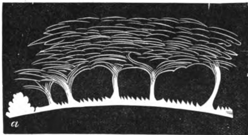
FIG. 122.—Tree-like prominences.
