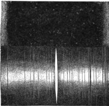
FIG. 52.—Non-coincidence of bright and dark F line when tangential slit is used, and when both photospheric and chromospheric light is admitted.
