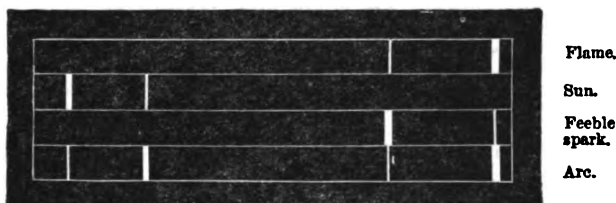
FIG. 92.—The various intensities of the lines of Lithium under different conditions.
