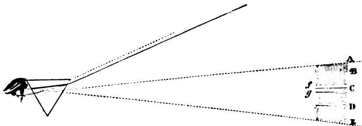
FIG. 5.—Copy of Wollaston's Diagram.
