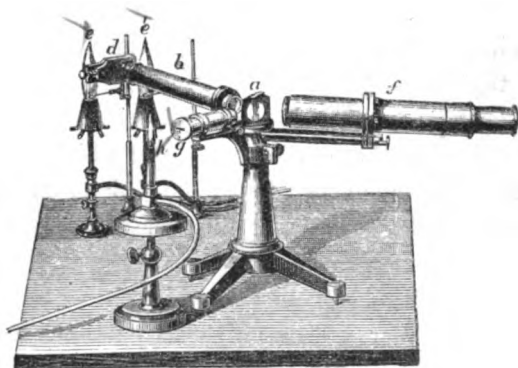
FIG. 28.—Spectroscope with reflected scale. a , prism; b , collimator; d , slit plate; e , e' , Bunsen burners for volatilising salts; f , observing telescope; g , photographic scale, illuminated by gas flame, h .
