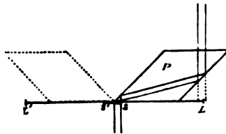
FIG. 40.—Mr. Hastings's arrangement for comparison of spectra. s s' , slit; l l' , diameter of sun's image; p , totally reflecting prism.
