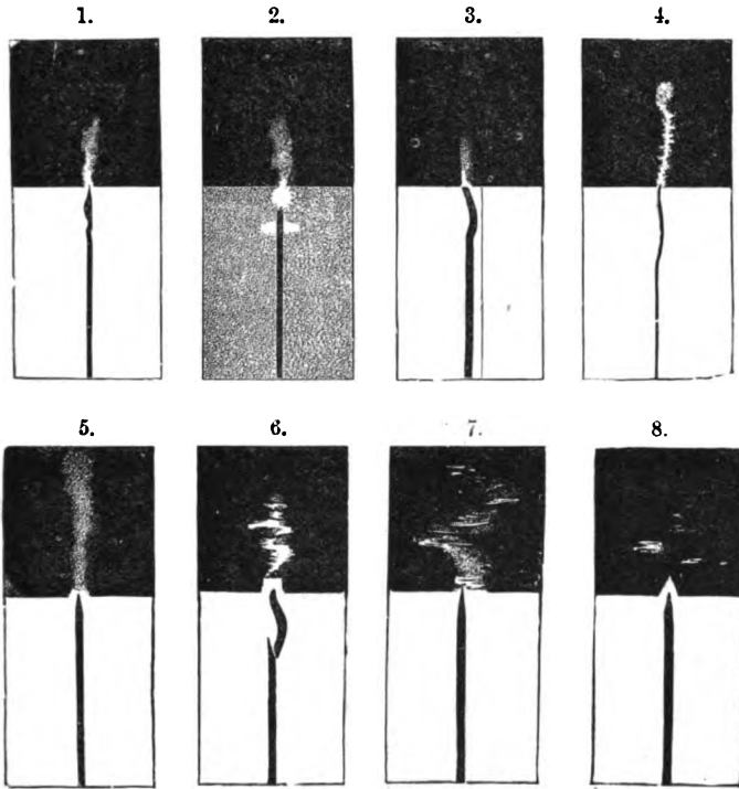
FIG. 58.—Motion forms and lozenges.
