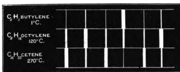
FIG. 98.—Hypothetical spectra obtained on distilling a successively increasing temperatures a mixture of light and heavy hydrocarbons.
