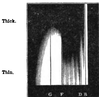
FIG. 18.—Absorption of sunlight by various thicknesses of a solution of the salts of chromium (Gladstone).
