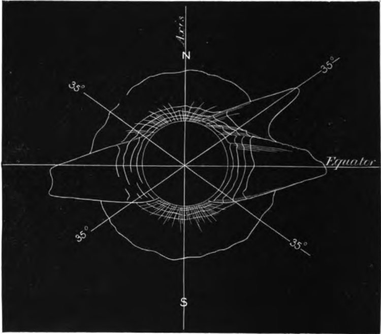
FIG. 134.—Tracing of the results obtained by the cameras in 1878, showing inner portion of equatorial extension, and how the surfaces of it cut the concentric atmosphere in lat. 35^\circ N. and S., or thereabouts.
