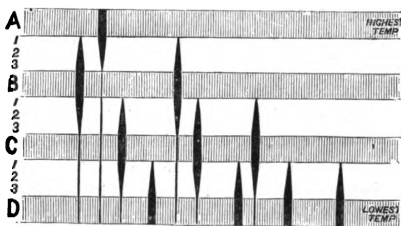
FIG. 86.—Hypothetical furnaces. The figures between the hypothetical spectra point to the gradual change in the intensities of the lines as the spectrum is observed near the temperature of each of the furnaces.
