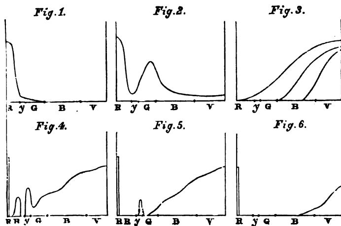
FIG. 16.—Copies of Herschel's Diagrams.
