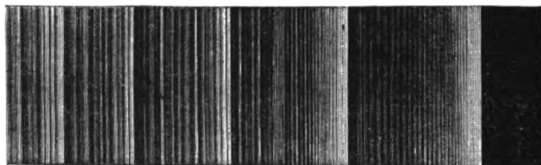
FIG 72.—Carbon flutings.
