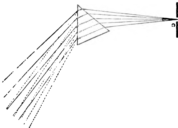
FIG. 8.—Showing arrangement of slit and prism (c slit).
