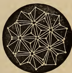
A molecule of Beryllium.
