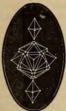
Nascent Hydride of Silicium.
