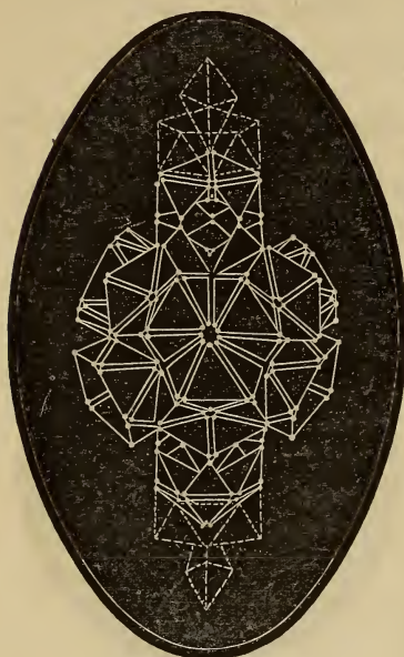
Monohydrated Nitric Acid (a bad diagram).
