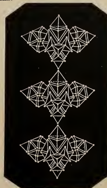
Sulphur Vapour, S^4 S^4 S^4
