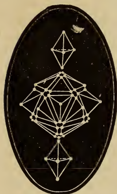
Hydride of Silicon (Nascent).
