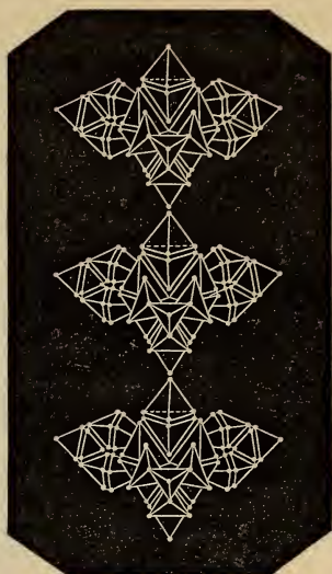
Sulphur Vapour, S^4S^4S^4 = \textcircled{S}^3 .
